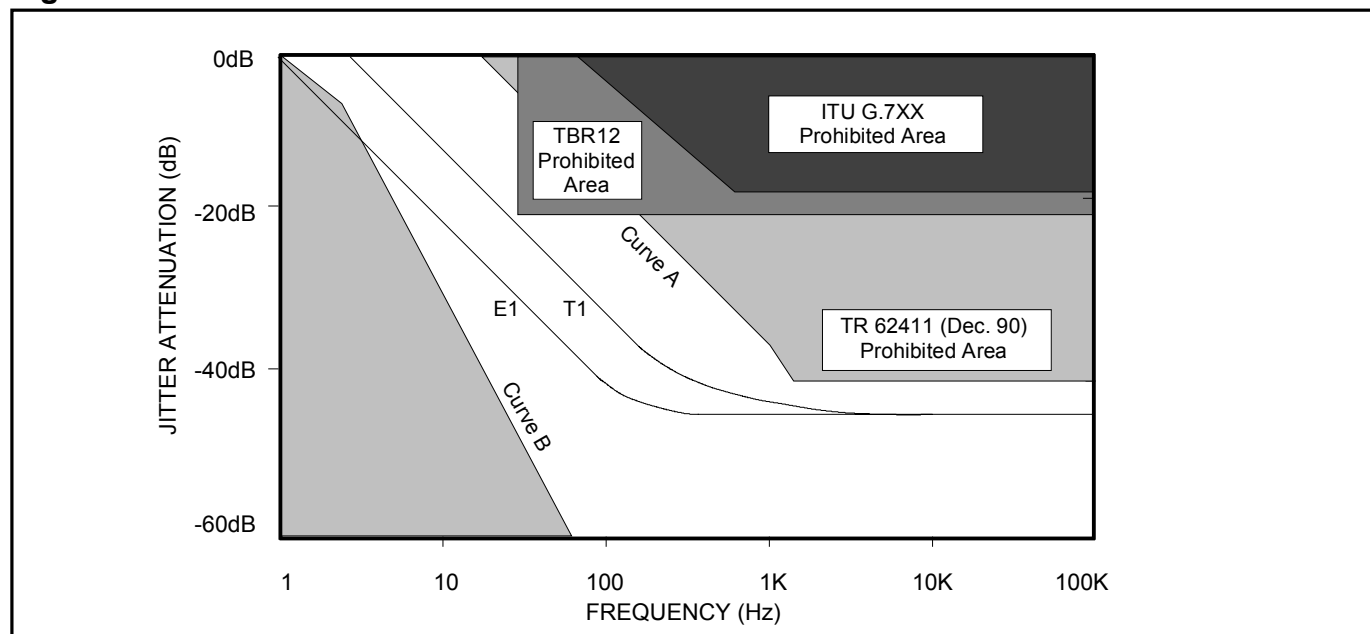
Figure 9-16. Jitter Attenuation
