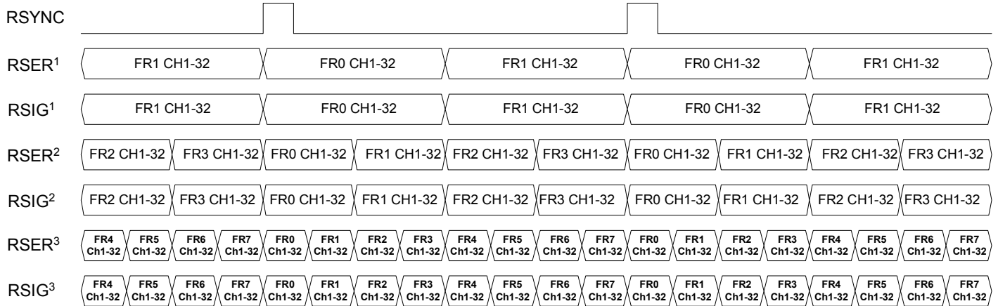
Figure 11-7. T1 Receive Side Interleave Bus Operation, FRAME Mode
