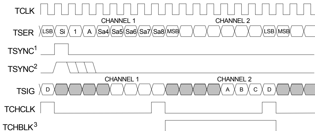
Figure 11-20. E1 Transmit Side Boundary Timing (elastic store disabled)
