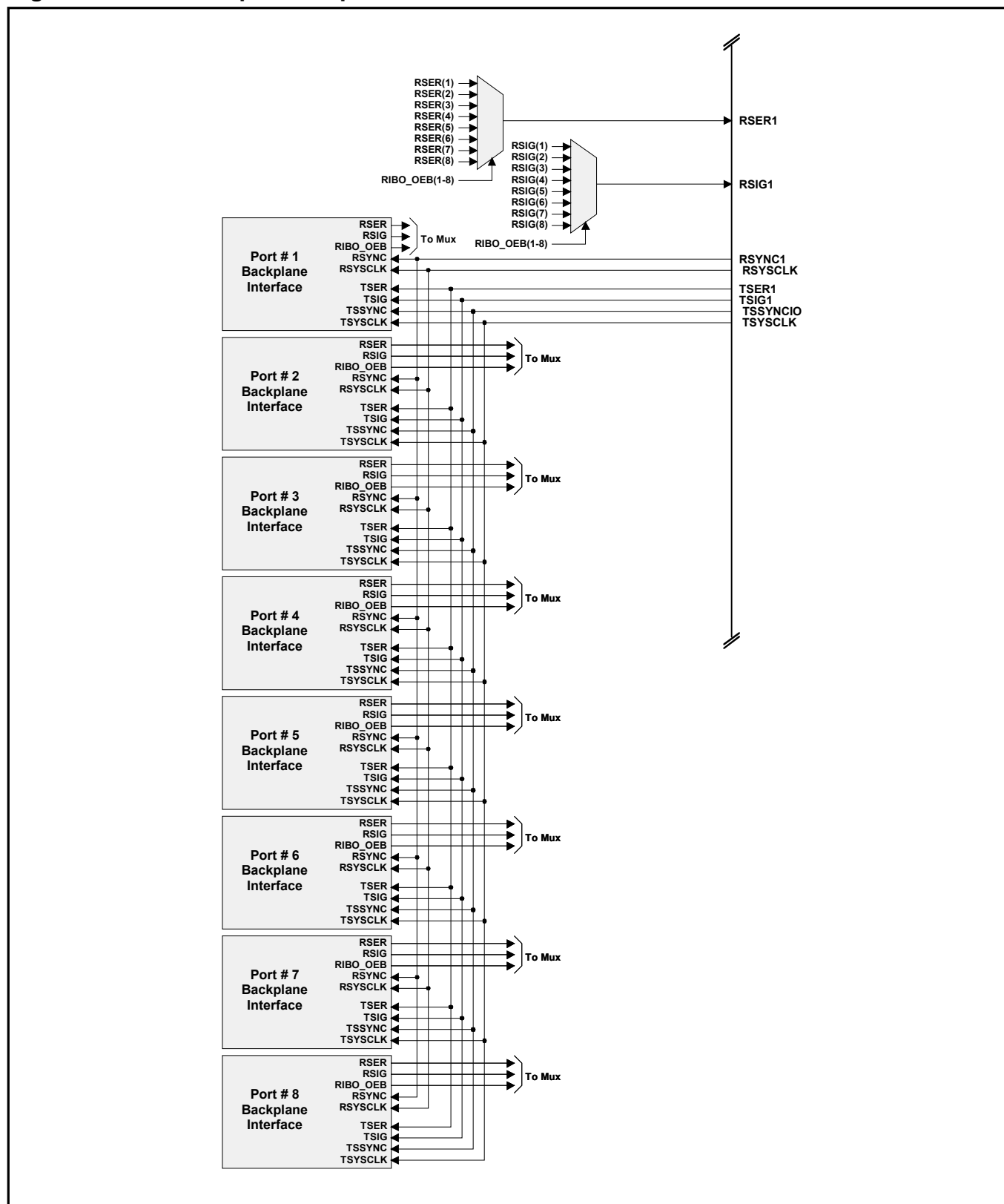
Figure 9-5. IBO Multiplexer Equivalent Circuit—16.384MHz
