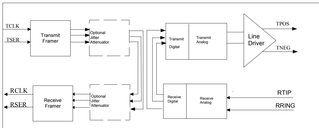
Figure 9-20. Dual Loopback
