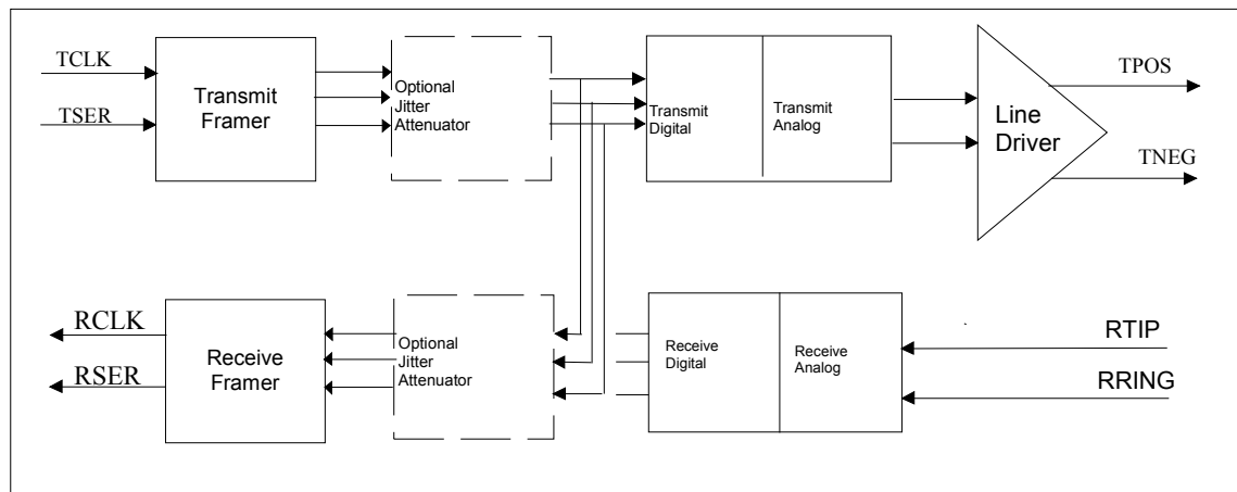
Figure 9-18. Local Loopback
