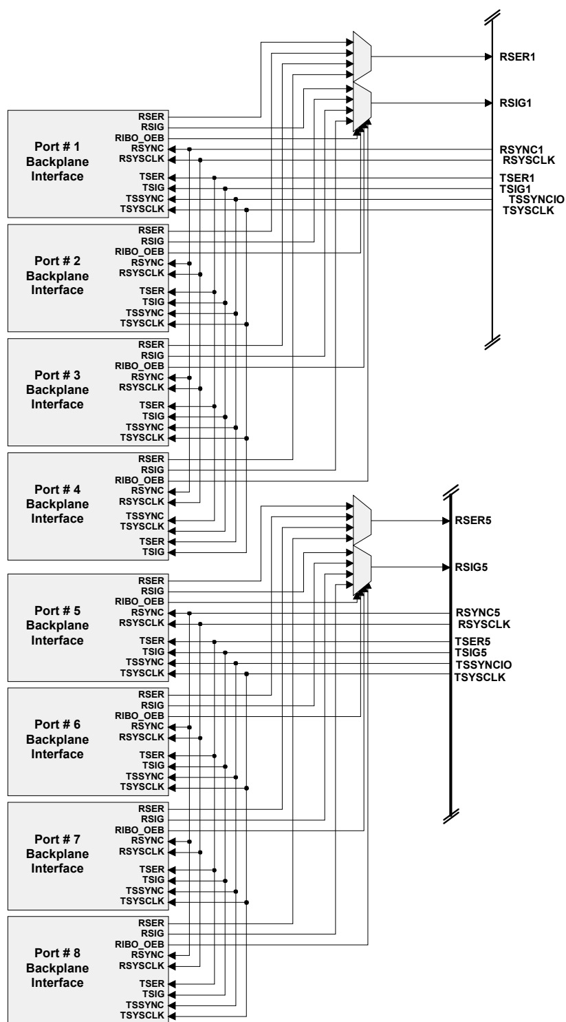
Figure 9-4. IBO Multiplexer Equivalent Circuit—8.192MHz
