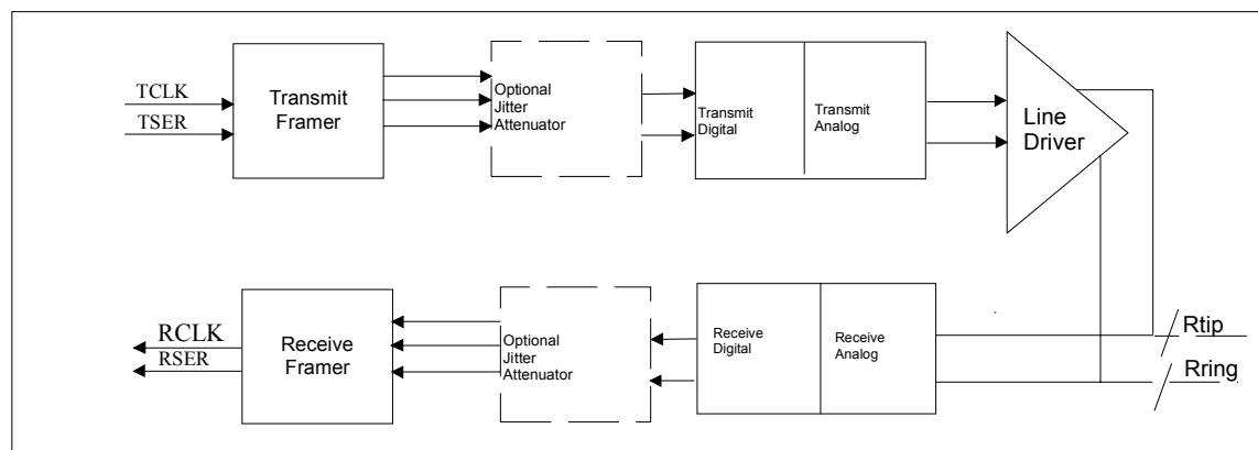
Figure 9-17. Analog Loopback
