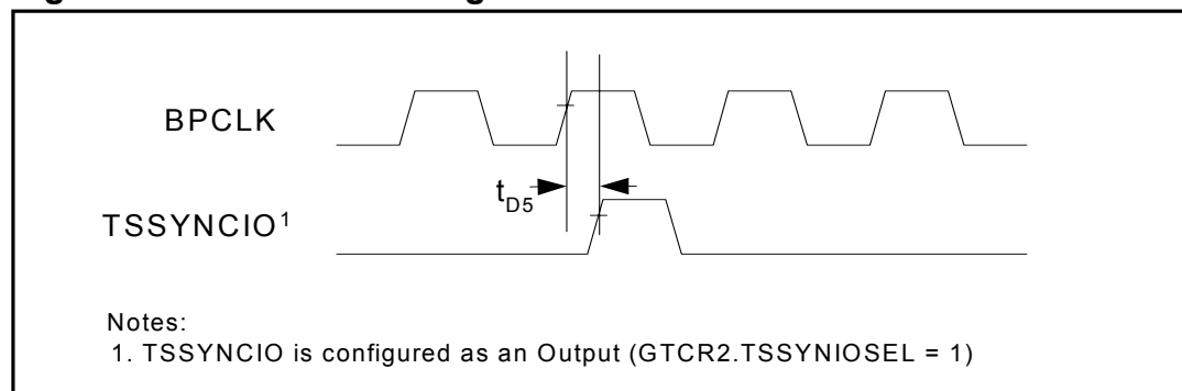
Figure 13-10. BPCLK Timing
