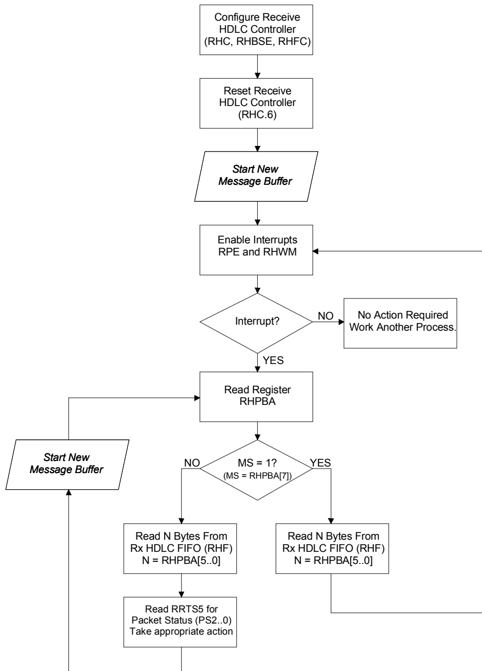
Figure 9-9. Receive HDLC Example
