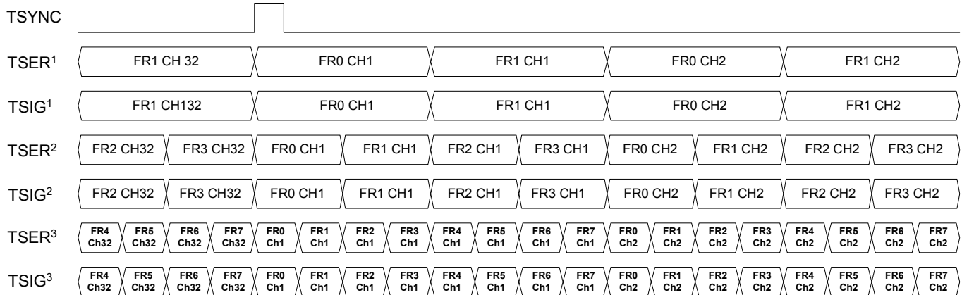
Figure 11-13. T1 Transmit Side Interleave Bus Operation, BYTE Mode
