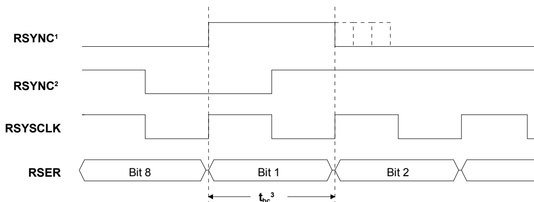
Figure 9-6. RSYNC Input In H.100 (Ct-Bus) Mode
