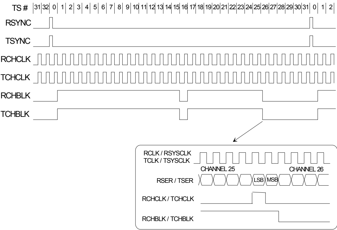
Figure 11-23. E1 G.802 Timing
