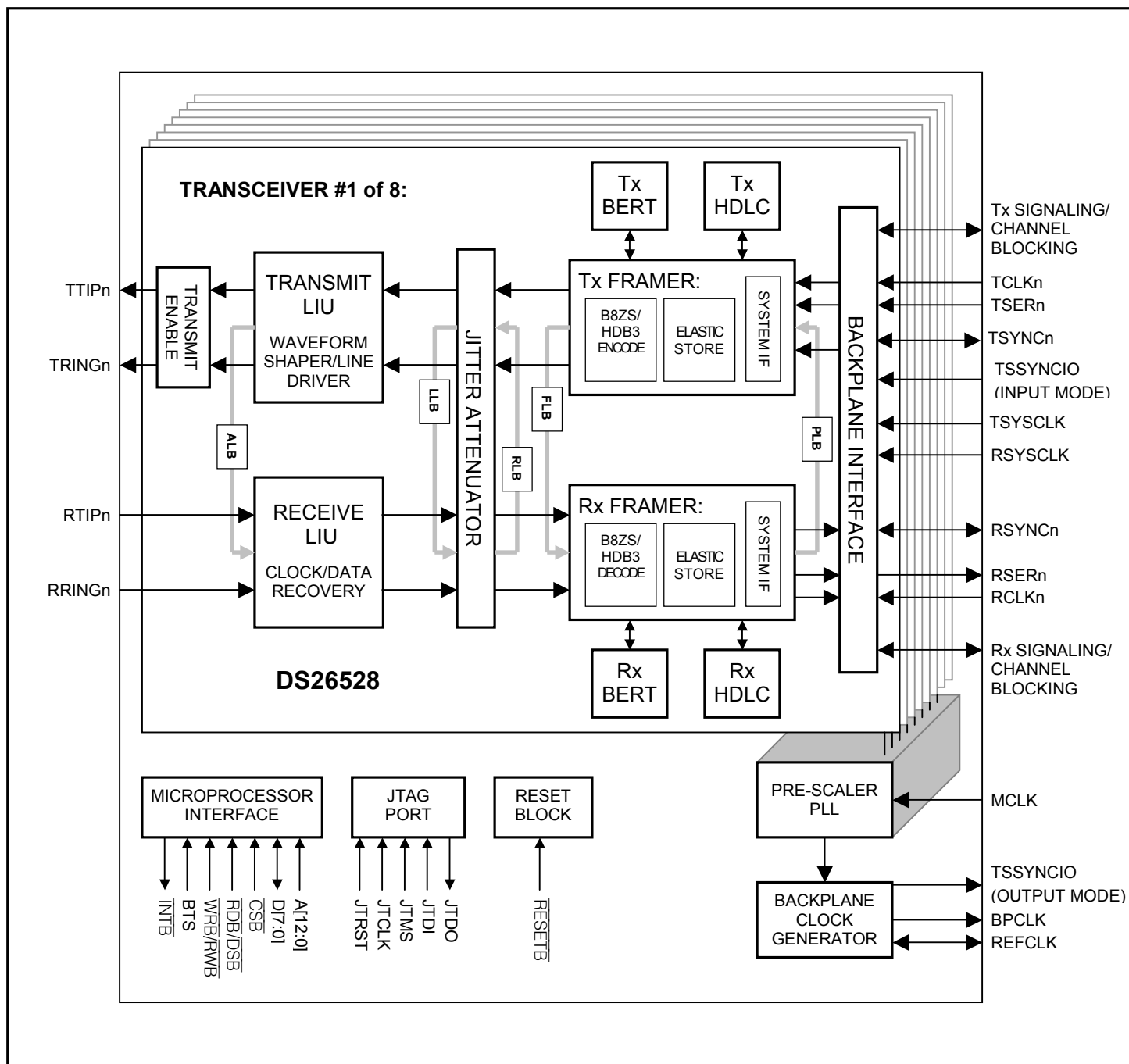
Figure 7-2. Detailed Block Diagram
