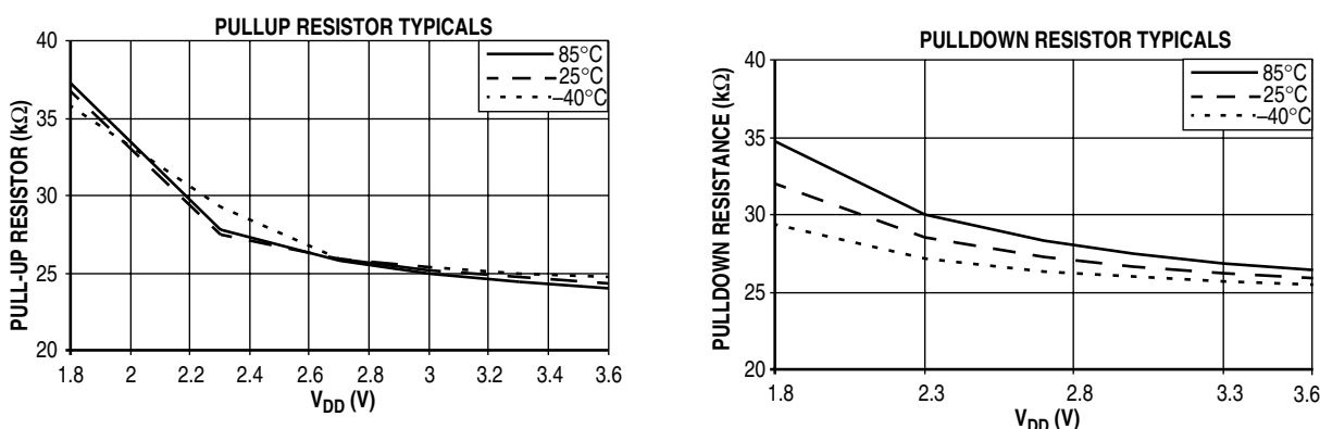
Figure A-1. Pullup and Pulldown Typical Resistor Values ( V_{DD} = 3.0 V)
