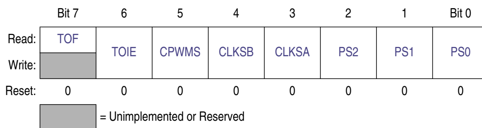
Figure 10-5. Timer x Status and Control Register (TPMxSC)
