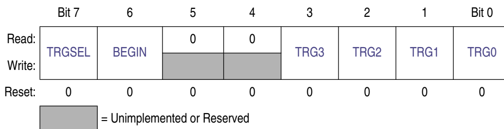
Figure 15-8. Debug Trigger Register (DBGT)
