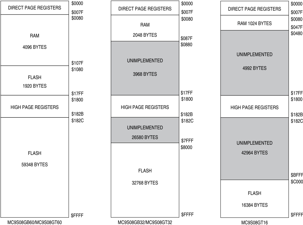
Figure 4-1. MC9S08GB/GT Memory Map
