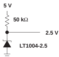
Figure 22. 2.5-V Reference
