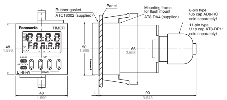
Pin type
