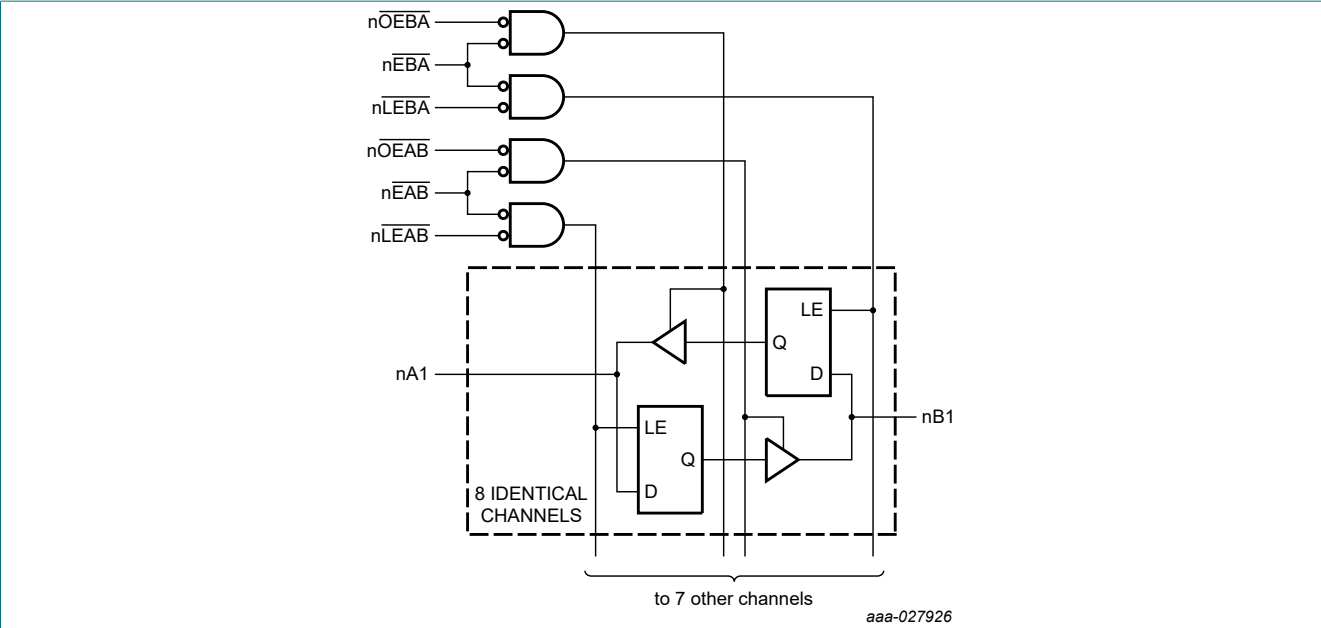
Fig. 3. Logic diagram
