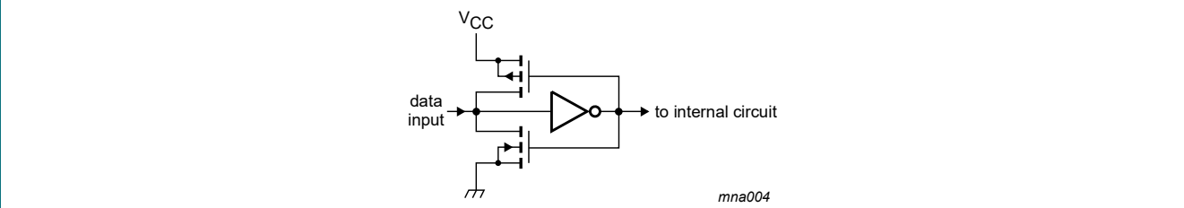
Fig. 4. Bushold circuit
