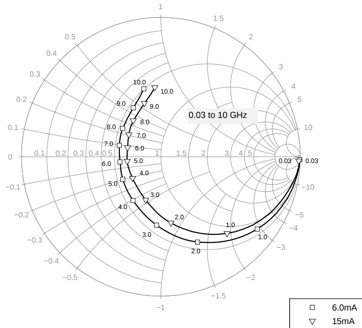
Figure 5-17 Output Matching S_{22} = f(f) , V_{CE} = 3\text{ V} , I_C = 6 / 15\text{ mA}
