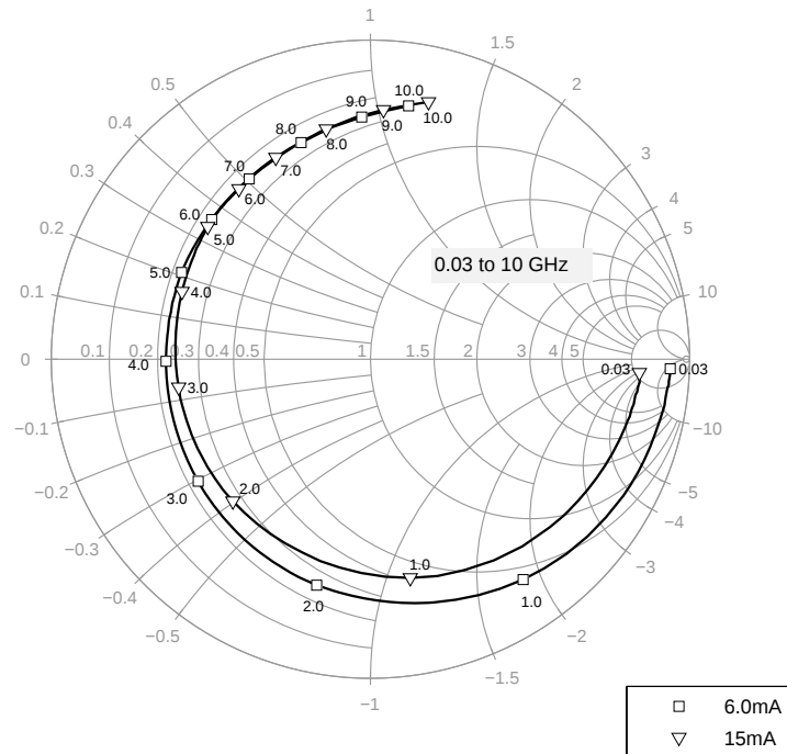
Figure 5-15 Input Matching S_{11} = f(f) , V_{CE} = 3\text{ V} , I_C = 6 / 15\text{ mA}
