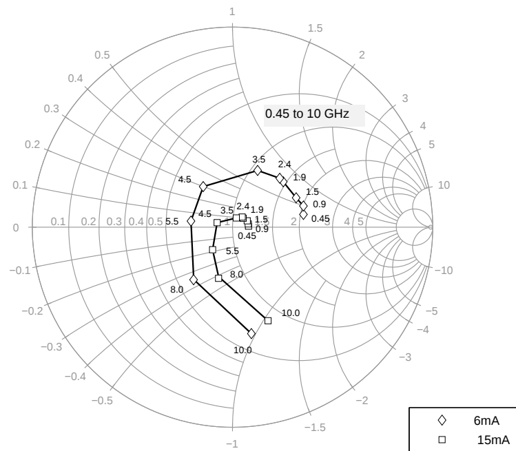
Figure 5-16 Source Impedance for Minimum Noise Figure Z_{opt} = f(f) , V_{CE} = 3\text{ V} , I_C = 6 / 15\text{ mA}
