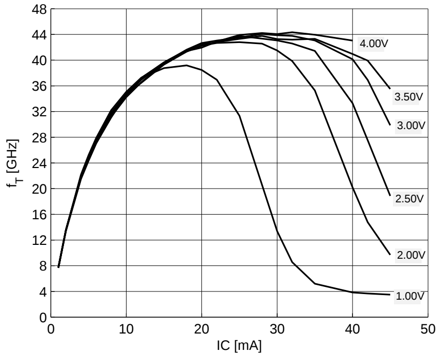
Figure 5-7 Transition Frequency f_T = f(I_C) , V_{CE} = \text{Parameter in V}
