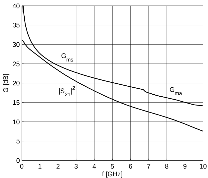
Figure 5-12 Gain G_{ma} , G_{ms} , |S_{21}|^2 = f(f) , V_{CE} = 3 V, I_C = 15 mA
