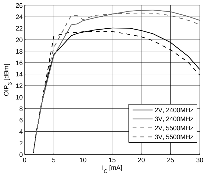
Figure 5-8 3rd Order Intercept Point at output OIP3 = f(I_C) , Z_S = Z_L = 50 \Omega , V_{CE}, f = \text{Parameters}
