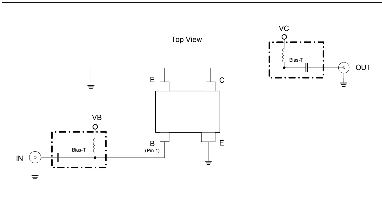
Figure 5-1 BFP740 Testing Circuit
