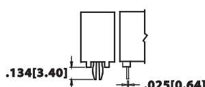
METAL BOARD LOCK (with no mounting ears) (R)
