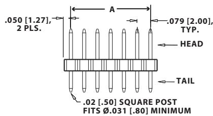
DUAL READOUT, STRAIGHT TAIL SHOWN
