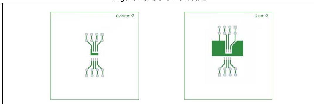
Figure 23. SO-8 PC board
