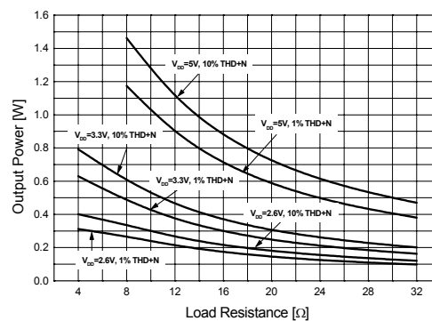
Figure 14. Output Power vs. Load Resistance
