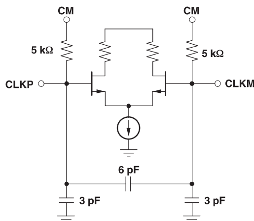
Figure 46. Clock Inputs
