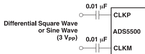
Figure 48. AC-Coupled, Differential Clock Input
