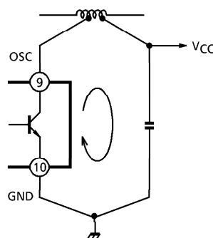
Fig.2 Oscillation Loop
