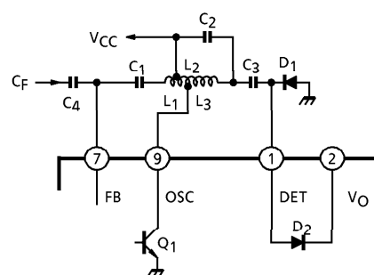
Fig.1 Oscillator and Voltage-Double
