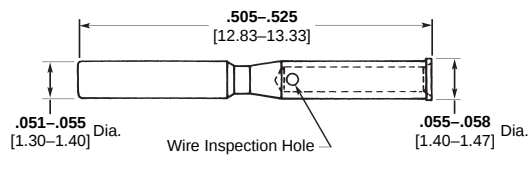
Part Number 082-0461-00Y9 (5-1532030-6) 22 AWG Socket
