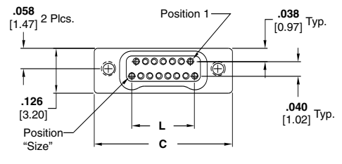
Receptacle with Flying Leads Drawing Number 1589476
