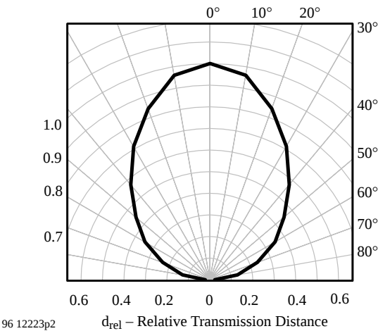
Figure 13. Directivity
