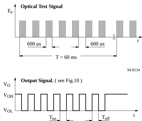
Figure 8. Output Function
