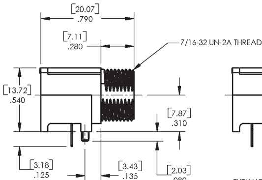
THRU HOLE TERMINATION SINGLE ROW (CONFIG. 3 & 4)
