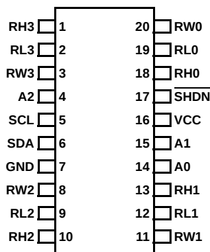
ISL22346 (20 LD TSSOP) TOP VIEW
