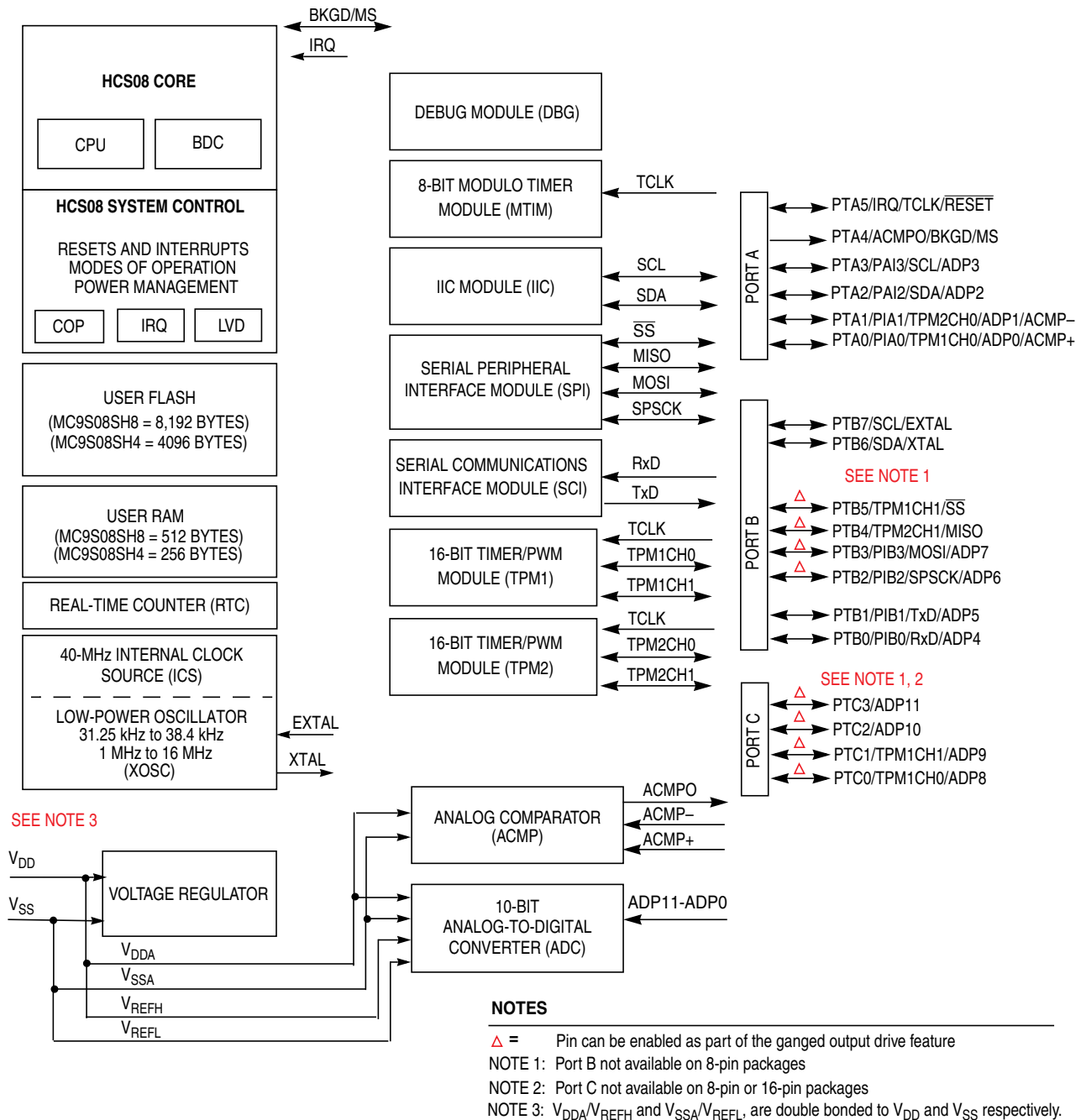
Figure 1-1. MC9S08SH8 Block Diagram
