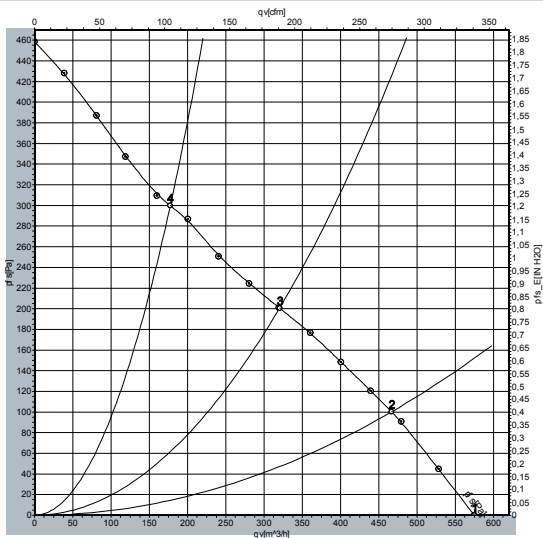
R2E190-RA50-21 Curves
