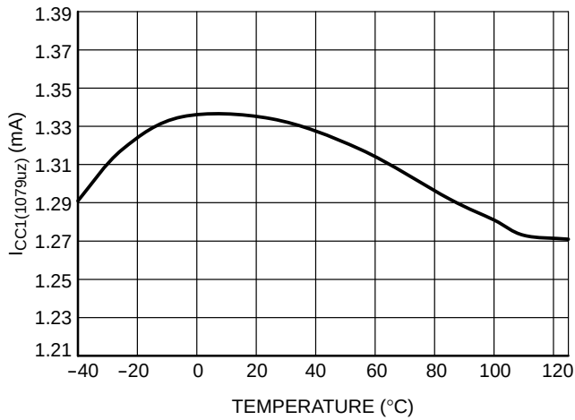
Figure 11. I_{CC1(0)1079uZ} vs. Temperature
