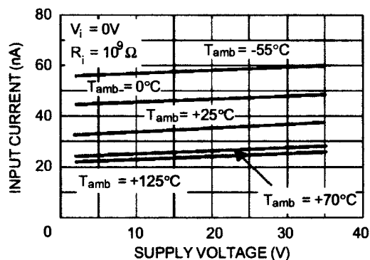
INPUT CURRENT versus SUPPLY VOLTAGE
