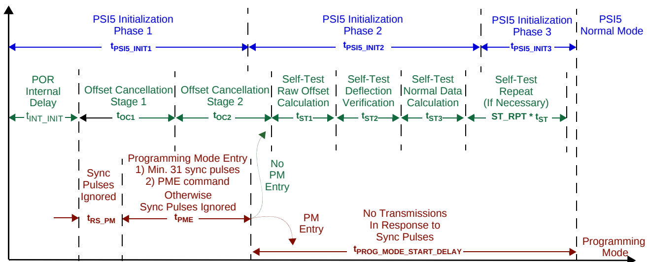
Figure 32. Initialization Timing
