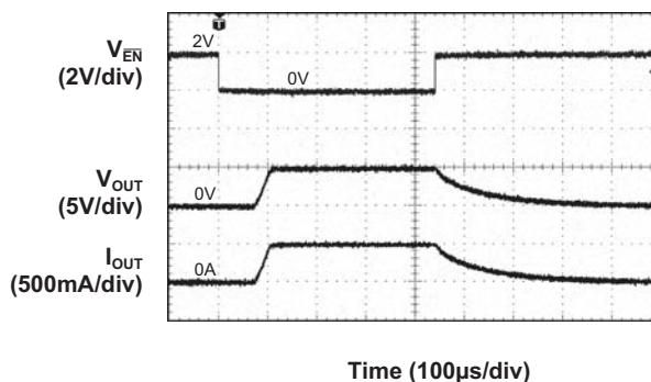
Turn-On/Off Response ( R_{OUT} = 10Ω ; V_{IN} = 5V )
