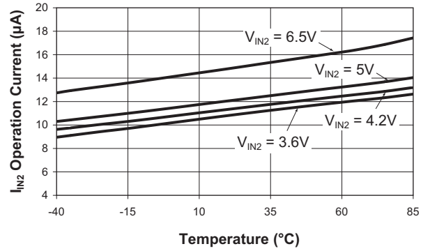
I_{IN2} Operation Current vs. Temperature ( I_{OUT} = 0A )
