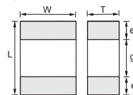
Chip Dimensions
