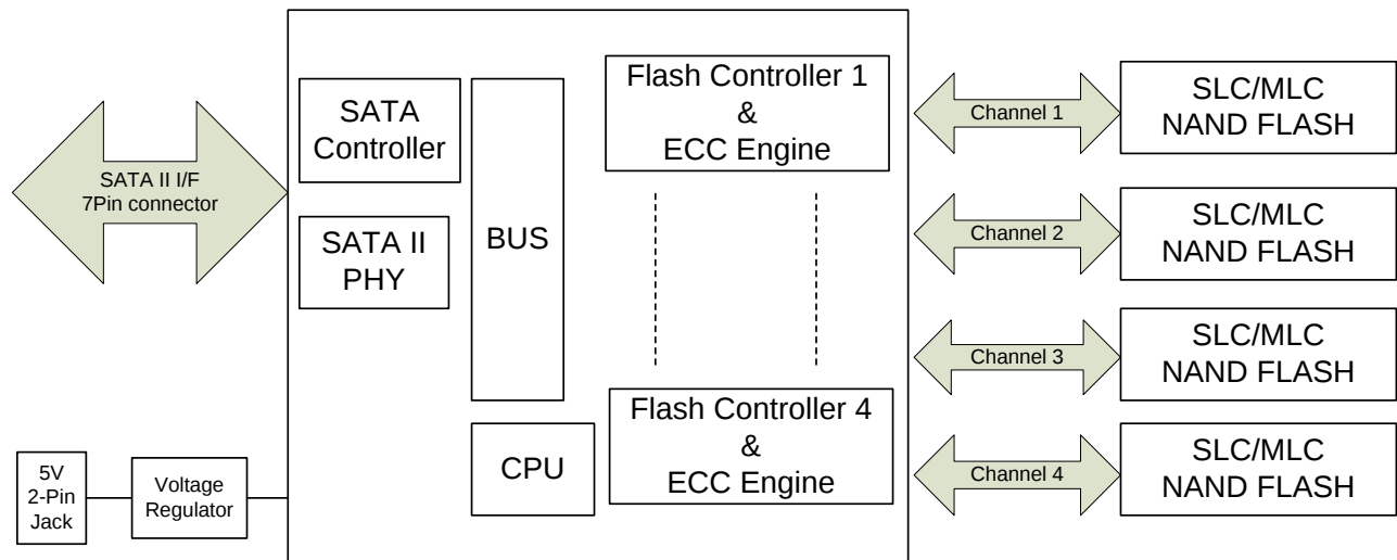
Figure 1. Block Diagram
