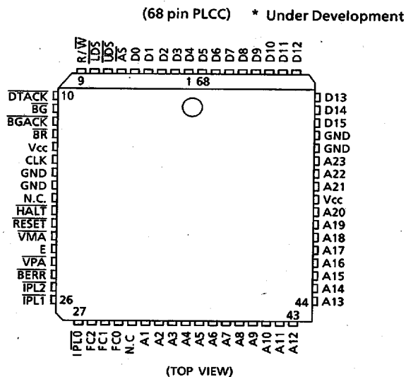
图 4.1 Input and Output Signals Pin Assignments (2/2)
