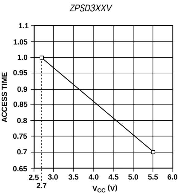
Figure 19. Normalized Access Time ( T_6 ) ( V_{CC} = 3.0\text{ V} )
