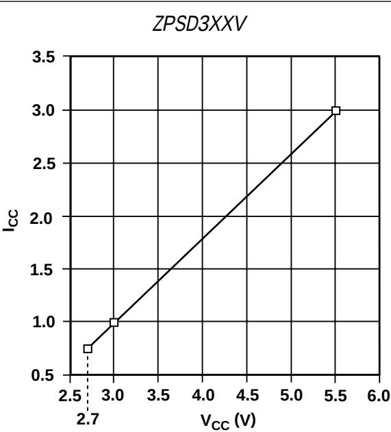
Figure 17. Normalized I_{CC} (DC vs. V_{CC} ) ( V_{CC} = 3.0\text{ V} )
