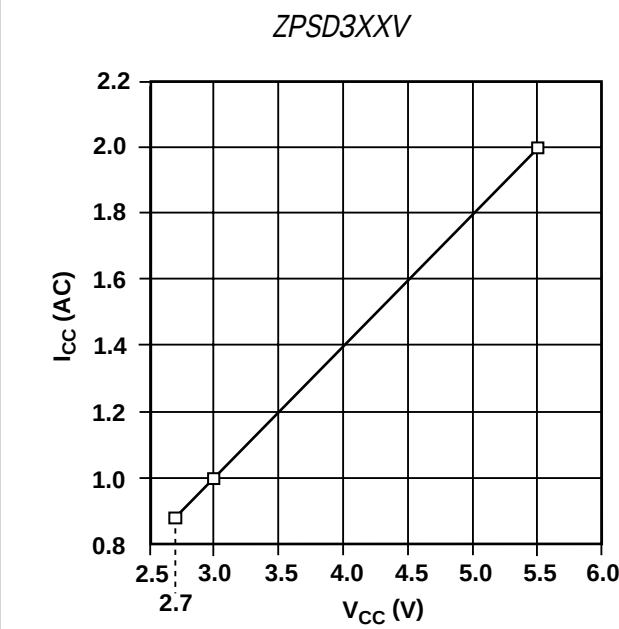
Figure 18. Normalized I_{CC} (AC) ( V_{CC} = 3.0\text{ V} )
