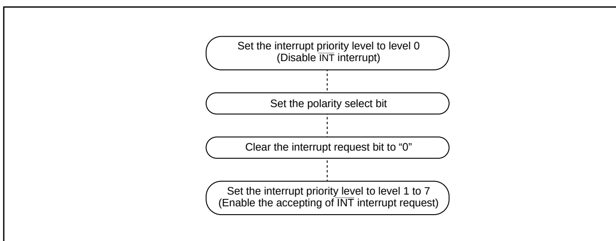
Figure 1.9.12. Switching condition of INT interrupt request
