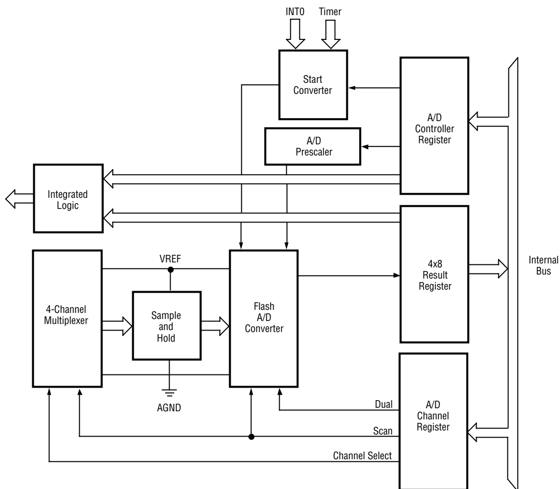
Figure 9. ADC Architecture
