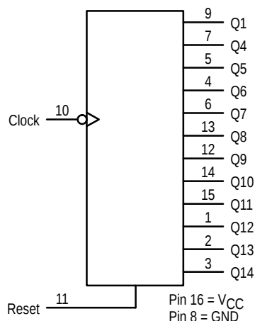
LOGIC DIAGRAM
