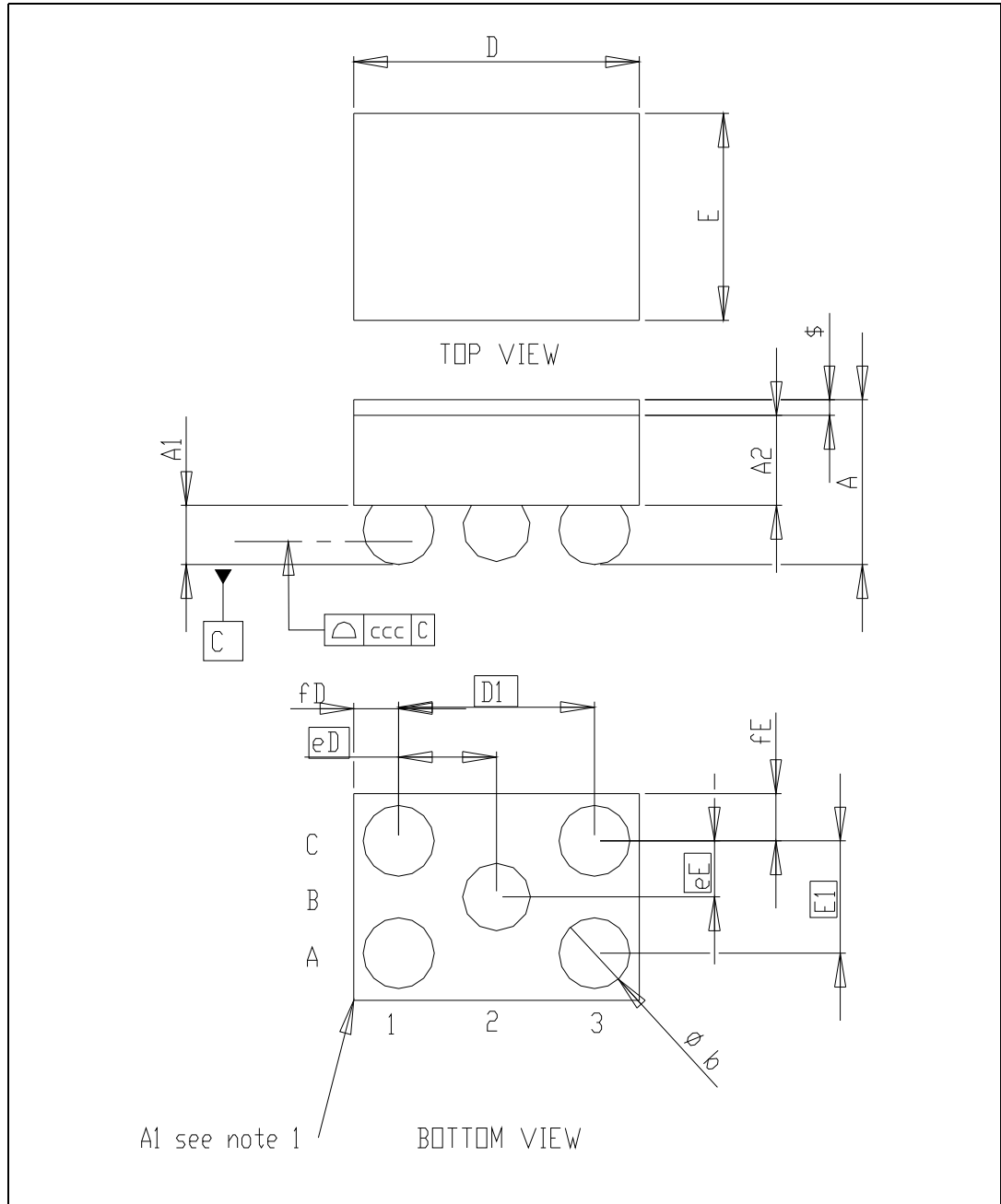
Figure 23. Flip-chip 5 drawings
