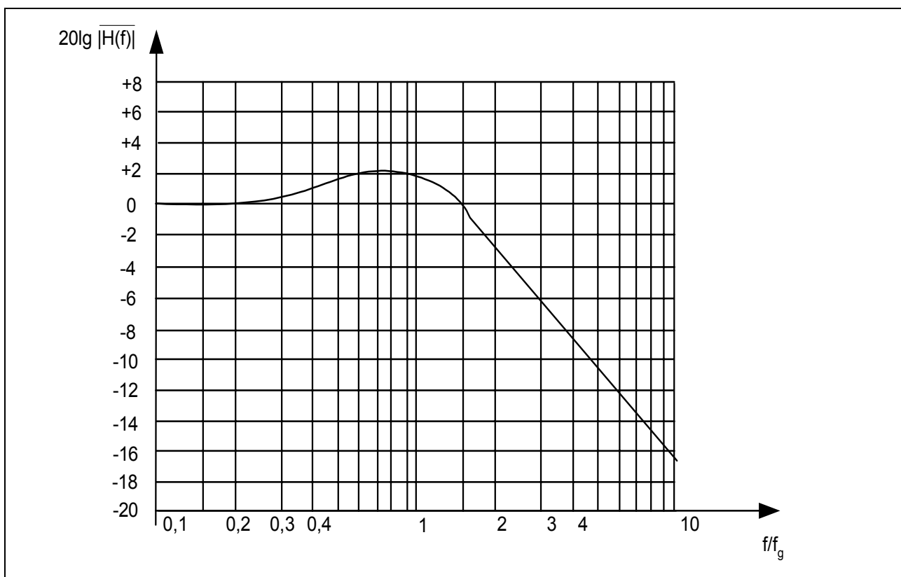
Figure 13 APLL - Jitter Transfer Function
