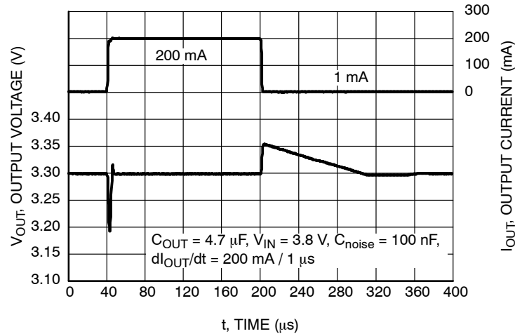
Figure 28. Load Transient Response, V_{OUT} = 3.3 V , C_{OUT} = 4.7 \mu F , C_{noise} = 100 nF
