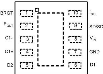
Figure 1. Top View 10-Lead WSON
