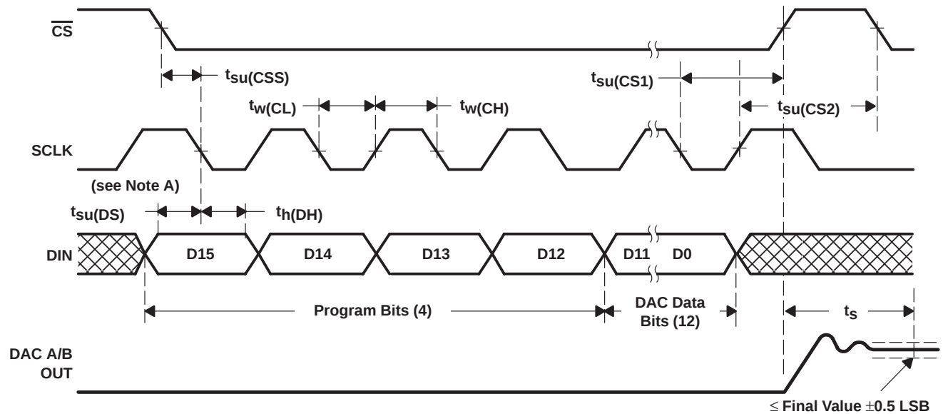
Figure 1. Timing Diagram for the TLC5618
