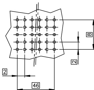
LAYOUT FOR P.C.B
