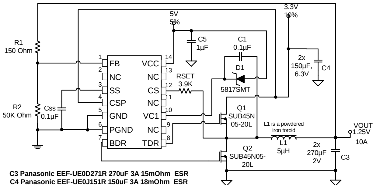
Figure 4 – 3.3V to 1.25V with Charge Pump.
