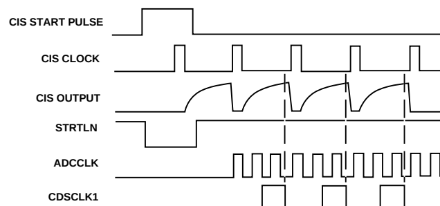
Figure 24. CIS Application Timing Signals
