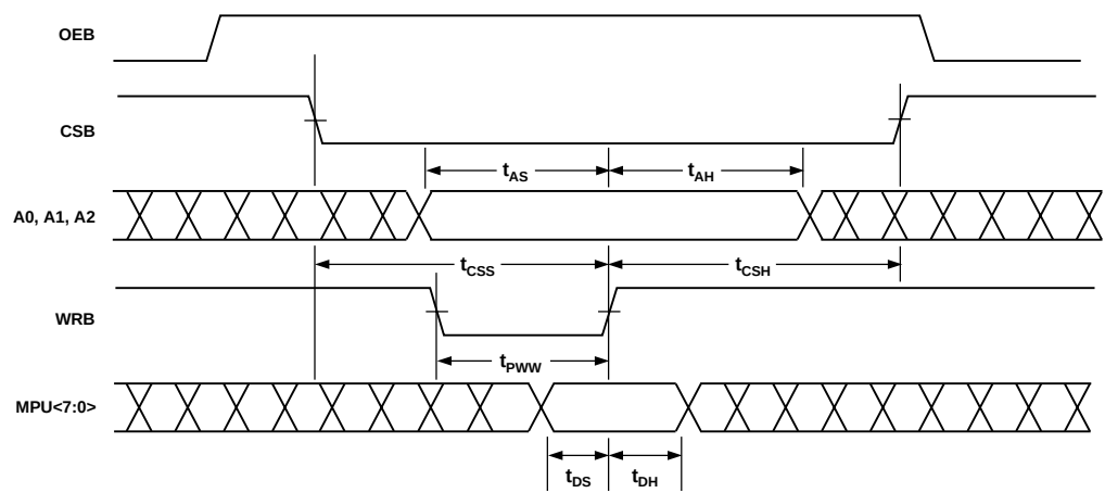
Figure 2. Write Timing
