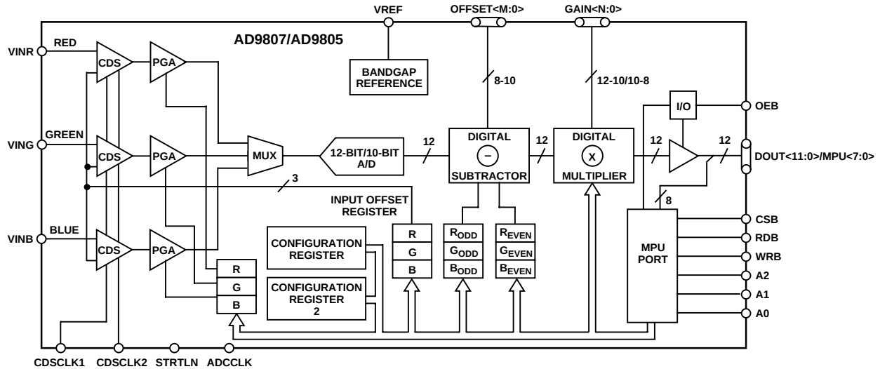
Figure 4. Block Diagram
