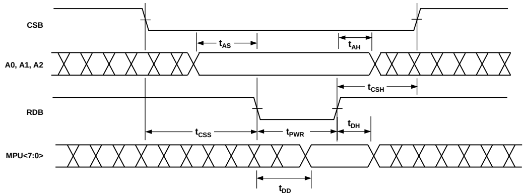
Figure 3. Read Timing
