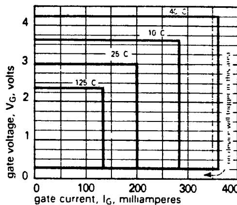
Figure 15 Gate triggering characteristics.
