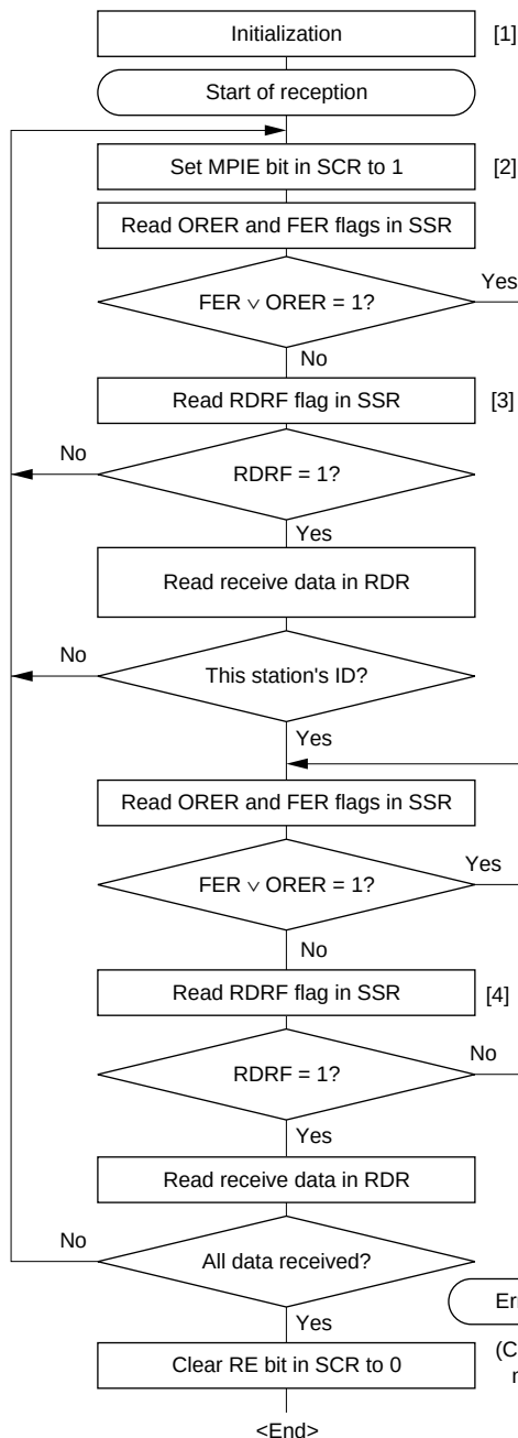
Figure 15.13 Sample Multiprocessor Serial Reception Flowchart (1)
