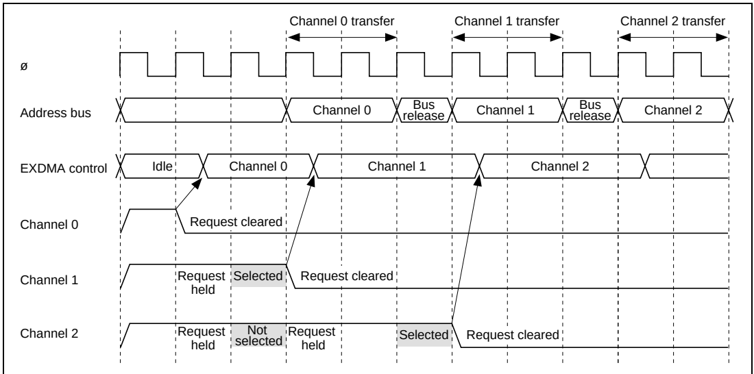
Figure 8.13 Example of Channel Priority Timing
