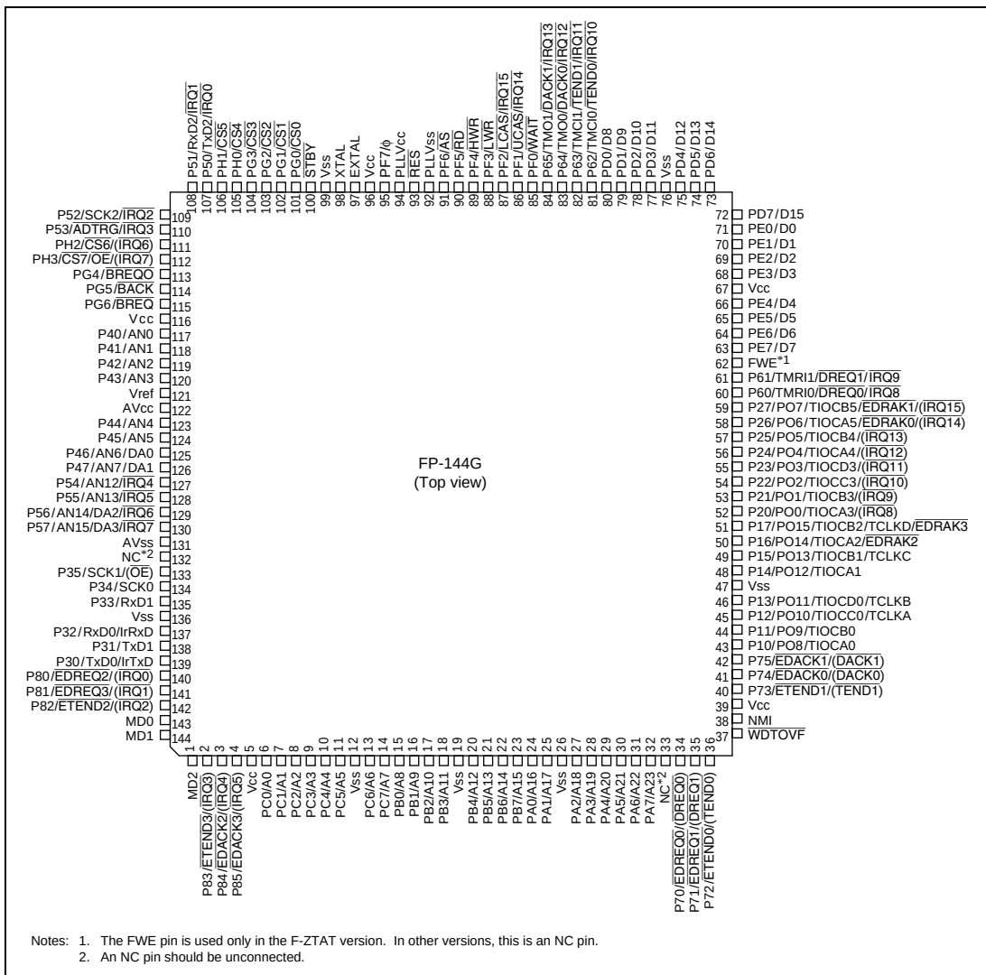
Figure 1.3 H8S/2678 Series Pin Arrangement
