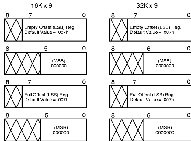
Figure 1. Offset Register Location and Default Values
