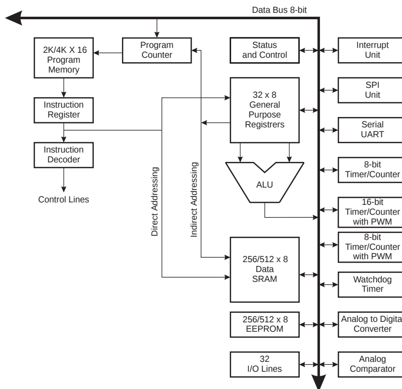
AVR AT90S4434/8535 Architecture
