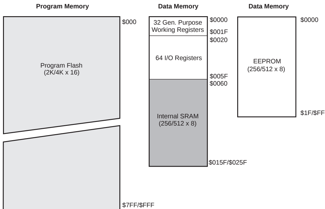
Figure 4. Memory Maps
