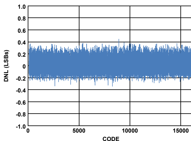
FIGURE 10. DIFFERENTIAL NONLINEARITY (250MSPS)
