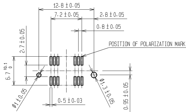
RECOMMENDED LAND PATTERN DIMENSION OF PCB (MOUNTING SIDE) (RECOMMENDED METAL MASK THICKNESS: 0.15mm)
