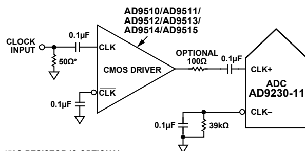
Figure 27. Single-Ended 1.8 V CMOS Sample Clock
