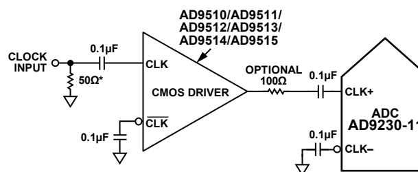
Figure 28. Single-Ended 3.3 V CMOS Sample Clock
