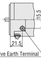
Detail Drawing of Protective Earth Terminal
