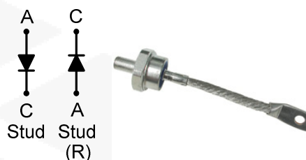
DO-8 Package
