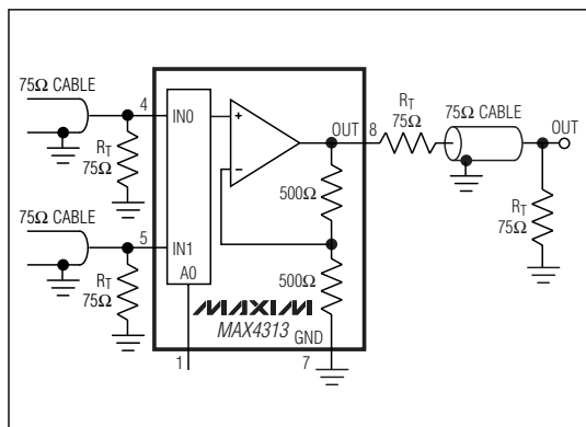
Figure 5. Video Line Driver
