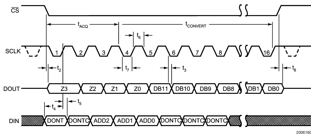
ADC78H89 Serial Timing Diagram
