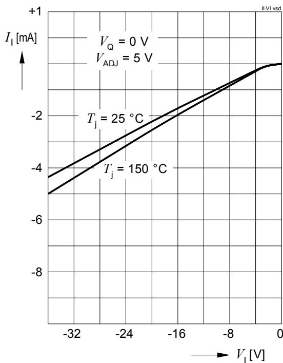
Reverse Current I_{\text{I}} vs. Input Voltage V_{\text{I}}
