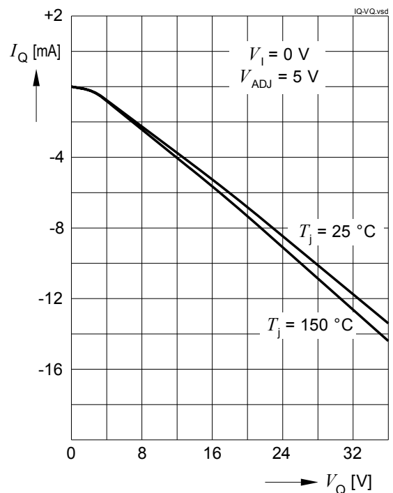
Reverse Output Current I_{\text{Q}} vs. Output Voltage V_{\text{Q}}
