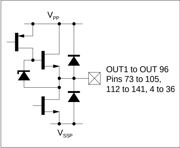
Figure 6: Power Output
