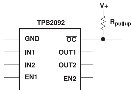
Figure 25. Typical Circuit for \overline{OC} Pin
